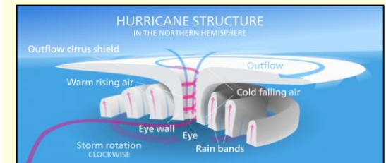
Structure of a hurricane
